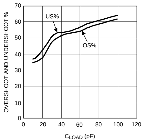
Figure 27. Overshoot and Undershoot vs C_{LOAD}
