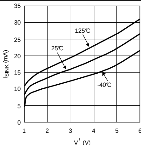
Figure 16. Sinking Current vs Supply Voltage
