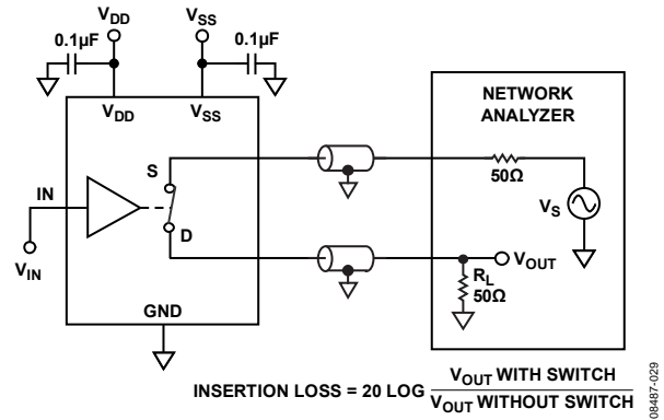
Figure 31. Bandwidth
