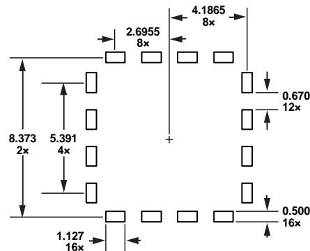
9.2mm x 9.2mm STACKED LGA PACKAGE
