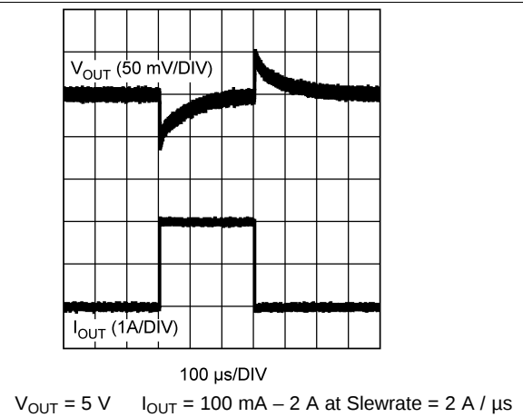
Figure 2. Load Transient See Figure 34
