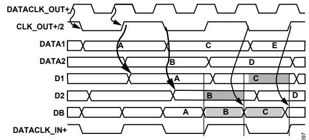
Figure 99. FPGA/ASIC Timing for Driving AD973x Digital Inputs, 2x Mode
