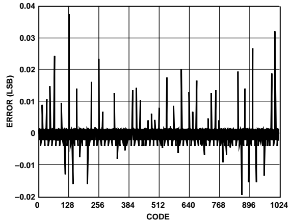
Figure 36. AD9734 DNL, 25°C, 10 mA FS
