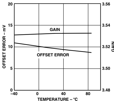
TPC 2. Offset Error and Gain vs. Temperature
