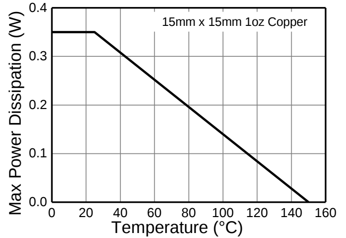
Figure 2. Derating Curve
