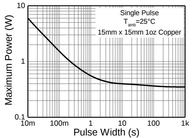
Figure 4. Pulse Power Dissipation
