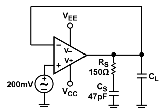
Figure 43. Snubber Network
