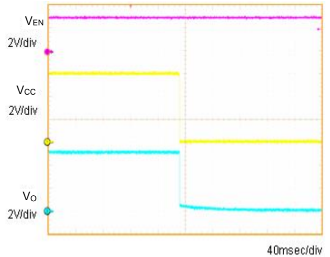
Fig.6 OFF sequence 1 Co=1µF
