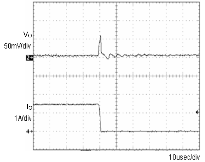
Fig.4 Transient Response (1.5→0A) Co=1µF
