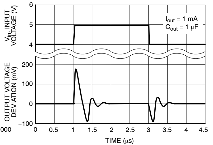
Figure 7. Line Transient Response
