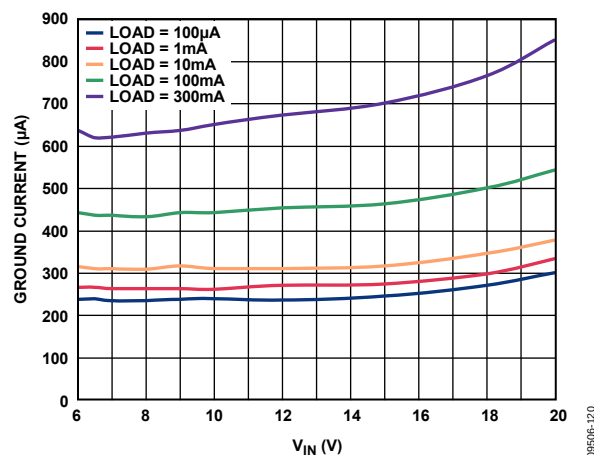
Figure 20. Ground Current vs. Input Voltage, V_{OUT} = 5\text{ V}
