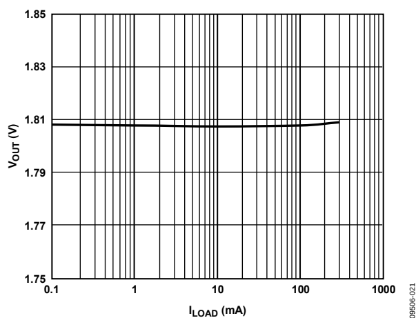
Figure 25. Output Voltage vs. Load Current, V_{OUT} = 1.8\text{ V}
