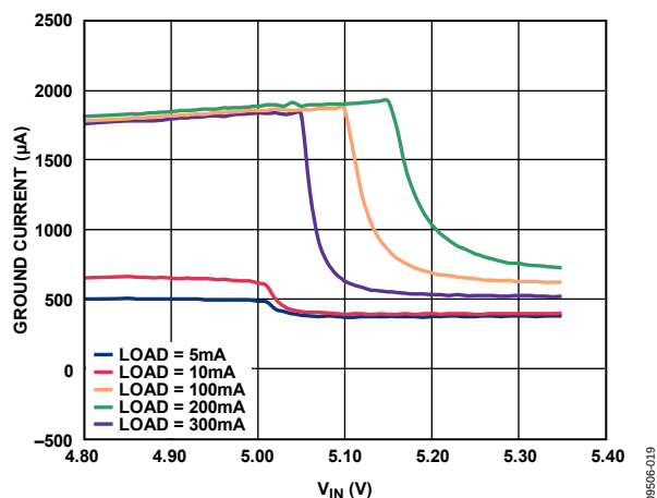
Figure 23. Ground Current vs. Input Voltage (in Dropout), V_{OUT} = 5\text{ V}
