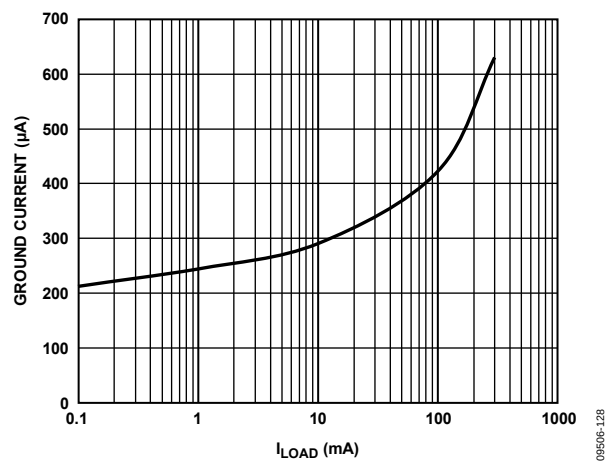
Figure 28. Ground Current vs. Load Current, V_{OUT} = 1.8\text{ V}
