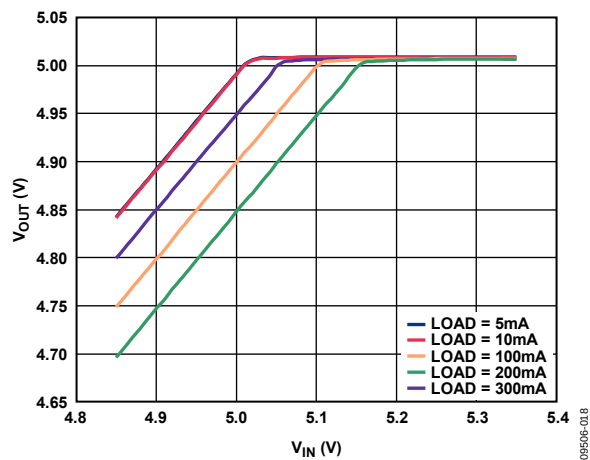
Figure 22. Output Voltage vs. Input Voltage (in Dropout), V_{OUT} = 5\text{ V}
