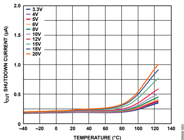
Figure 33. Reverse Input Current vs. Temperature, V_{IN} = 0\text{ V} , Different Voltages on V_{OUT}
