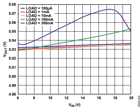
Figure 32. Output Voltage vs. Input Voltage, V_{OUT} = 5\text{ V} , Adjustable
