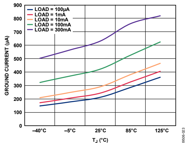
Figure 27. Ground Current vs. Junction Temperature, V_{OUT} = 1.8\text{ V}
