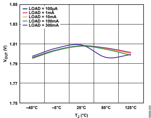
Figure 24. Output Voltage vs. Junction Temperature, V_{OUT} = 1.8\text{ V}
