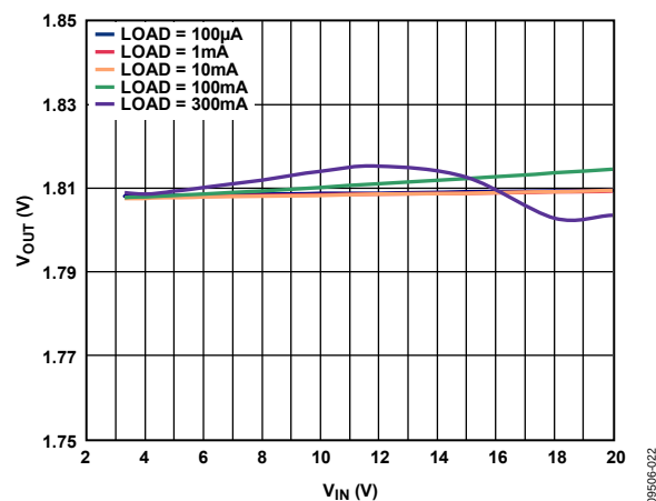
Figure 26. Output Voltage vs. Input Voltage, V_{OUT} = 1.8\text{ V}
