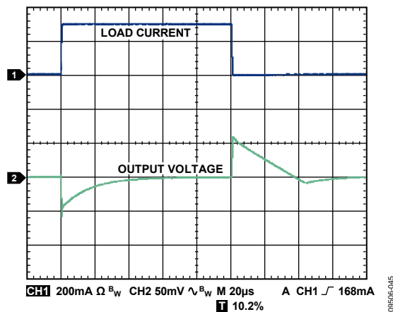
Figure 52. Load Transient Response, C_{IN} , C_{OUT} = 1\text{ }\mu\text{F} , I_{LOAD} = 1\text{ mA to }300\text{ mA} , V_{OUT} = 3.3\text{ V} , V_{IN} = 5\text{ V}
