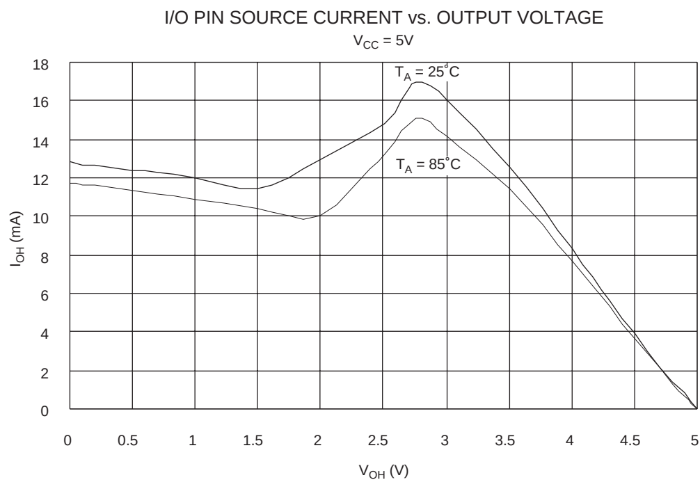
Figure 85. I/O Pin Source Current vs. Output Voltage
