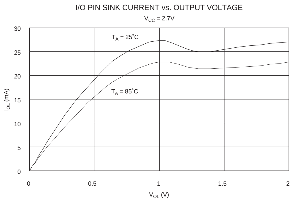
Figure 86. I/O Pin Sink Current vs. Output Voltage
