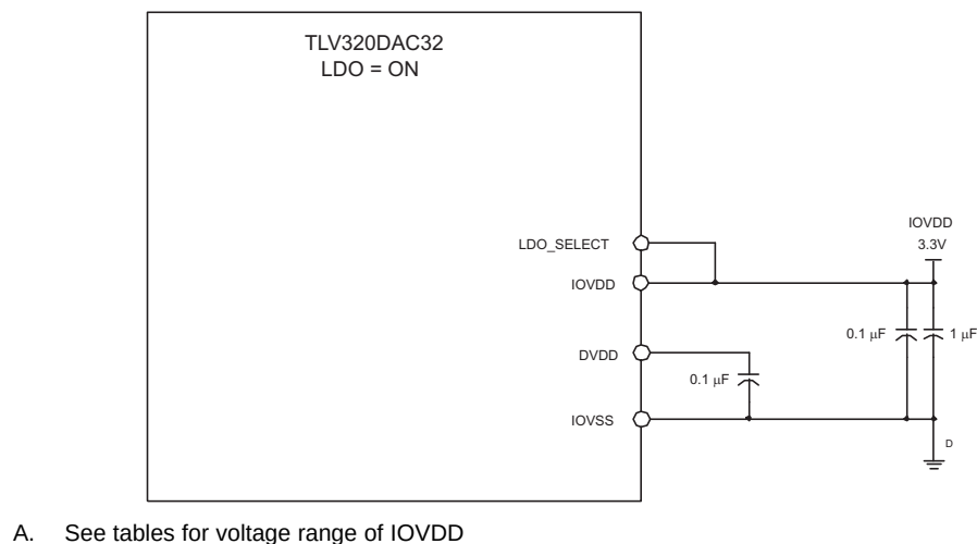
Figure 21. LDO Function Operating
