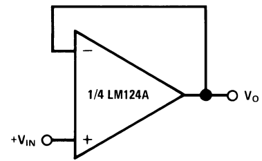
Figure 25. Voltage Follower
