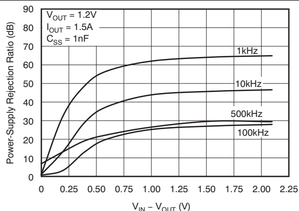
Figure 27. V_{IN} PSRR vs (V_{IN} - V_{OUT})
