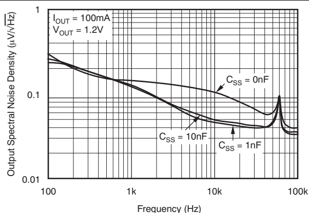
Figure 28. Noise Spectral Density
