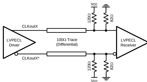
Figure 20. Differential LVPECL Operation, DC Coupling, Thevenin Equivalent
