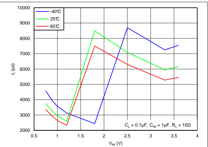
Figure 14. Rise Time vs Input Voltage (CL = 0.1 µF, RL = 10 Ω, VON = 1.8 V)
