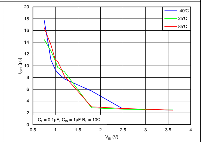
Figure 16. Turnoff Time vs Input Voltage (CL = 0.1 µF, RL = 10 Ω, VON = 1.8 V)
