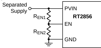
Figure 4. Resistor Divider for PVIN UVLO Setting
