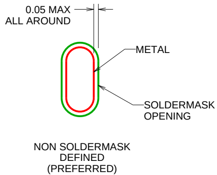
SOLDERMASK DETAILS
