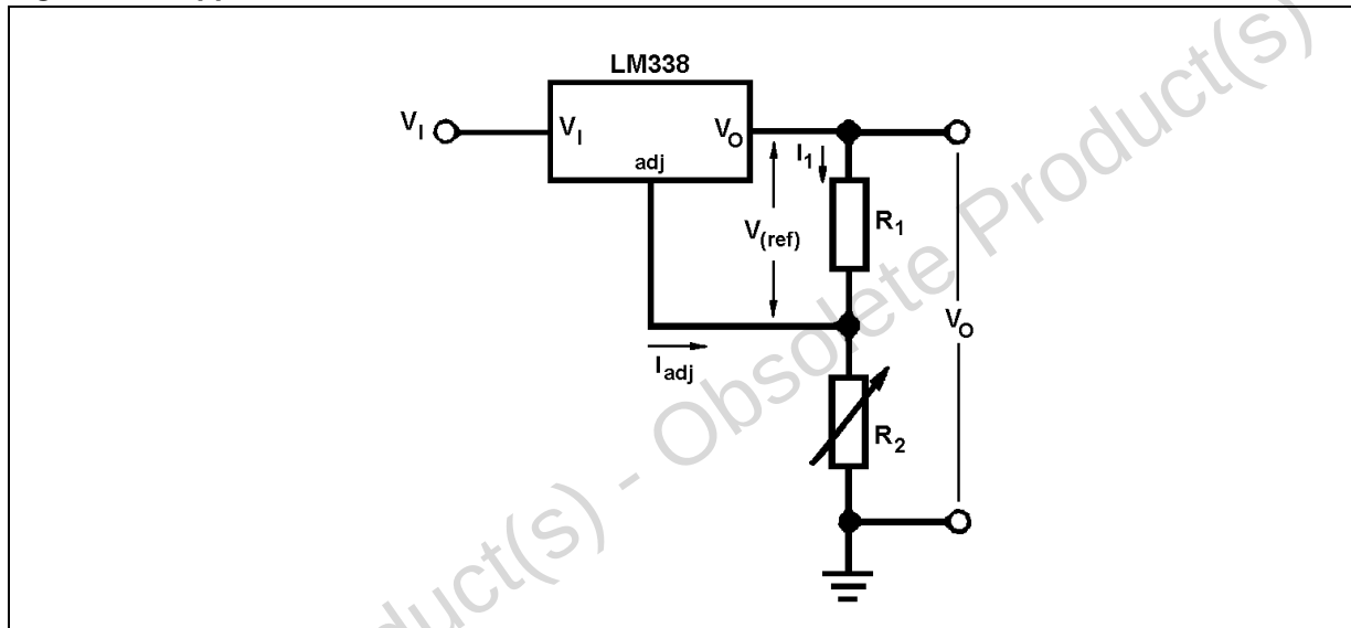
Figure 18. Application circuit
