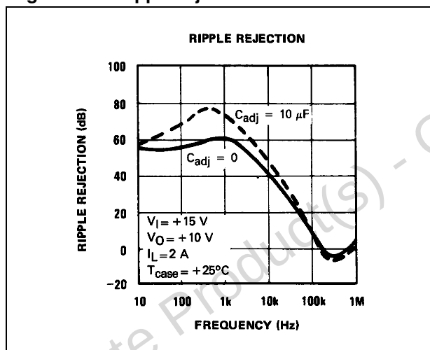
Figure 13. Ripple rejection
