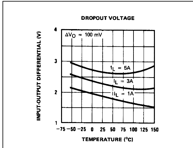
Figure 7. Dropout voltage
