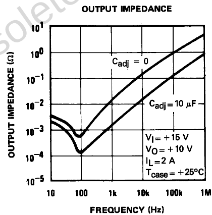
Figure 10. Output impedance
