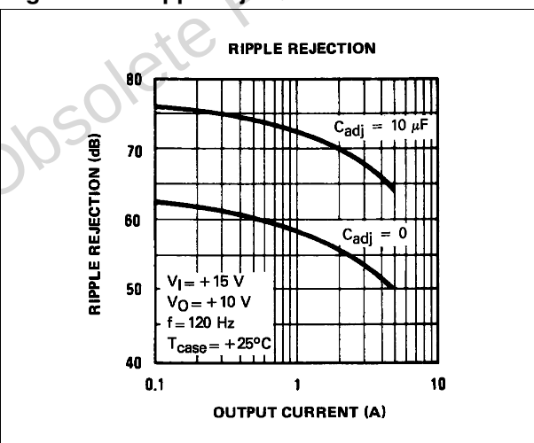
Figure 14. Ripple rejection
