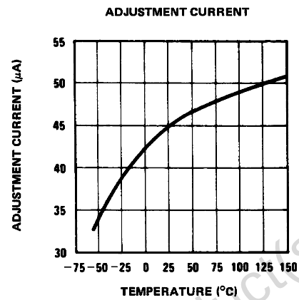
Figure 8. Adjustment current
