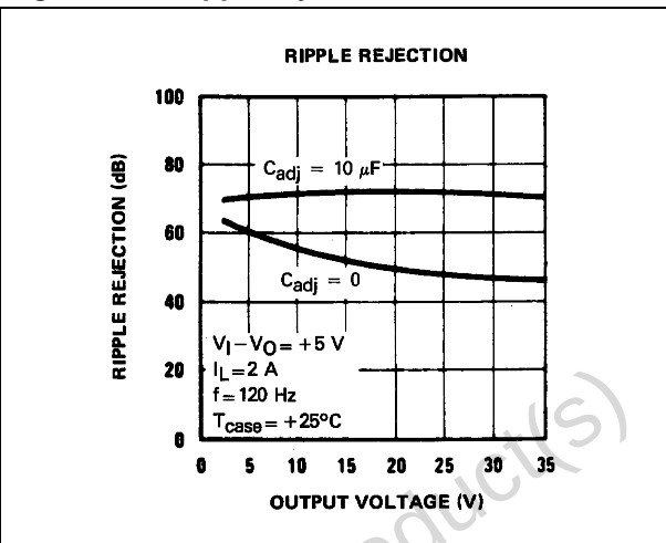
Figure 12. Ripple rejection
