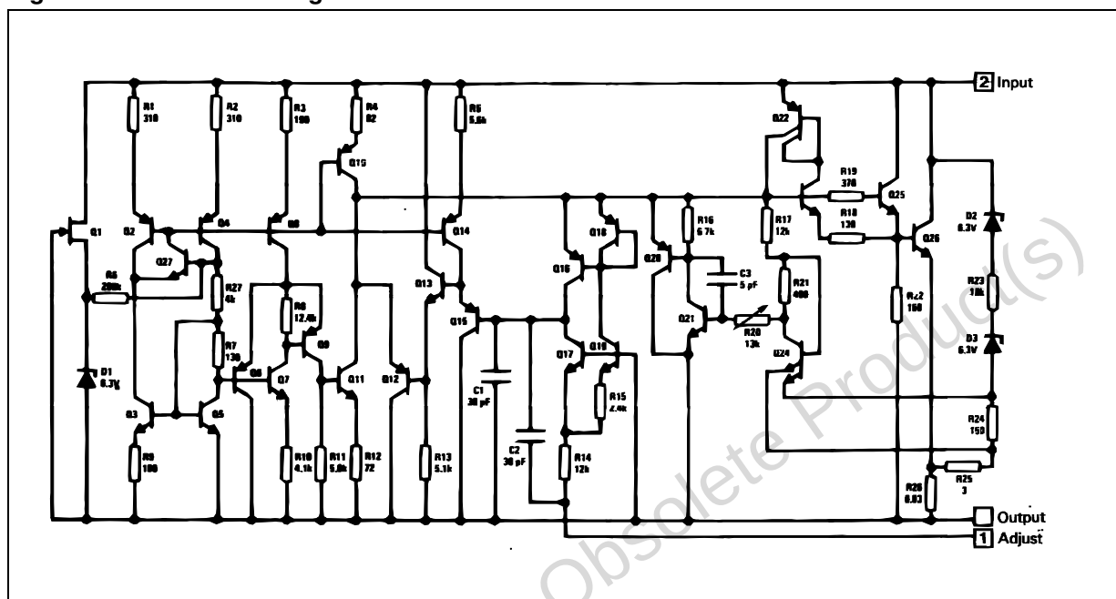
Figure 1. Schematic diagram
