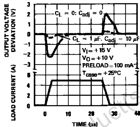
Figure 16. Load transient response
