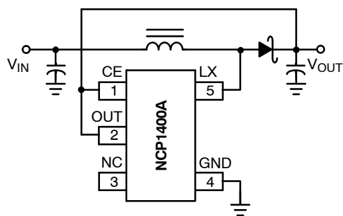
Figure 1. Typical Step-Up Converter Application
