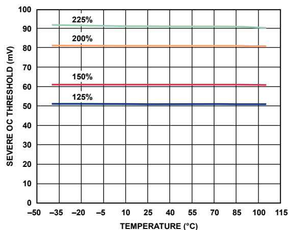
Figure 36. Severe OC Threshold vs. Temperature, ADM1075-2 , I_{SET} = 1.65\text{ V}
