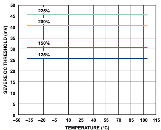
Figure 35. Severe OC Threshold vs. Temperature, ADM1075-1 , I_{SET} = 1.65\text{ V}
