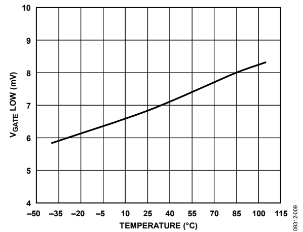
Figure 9. V_{GATE\ Low} vs. Temperature ( I_{GATE} = 100\ \mu\text{A} )
