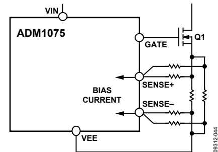
Figure 45. Connection of Multiple Sense Resistors to SENSE± Pins
