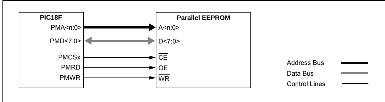
FIGURE 11-30: PARALLEL EEPROM EXAMPLE (UP TO 15-BIT ADDRESS, 8-BIT DATA)
