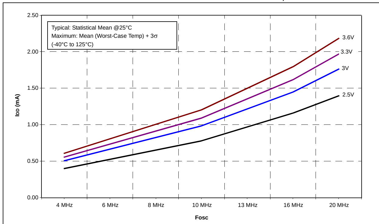
FIGURE 24-10: PIC16LF722/3/4/6/7 MAXIMUM I_{DD} vs. F_{OSC} OVER V_{DD} , HS MODE
