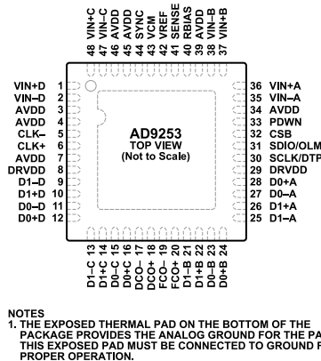
Figure 9. 48-Lead LFCSP Pin Configuration, Top View
