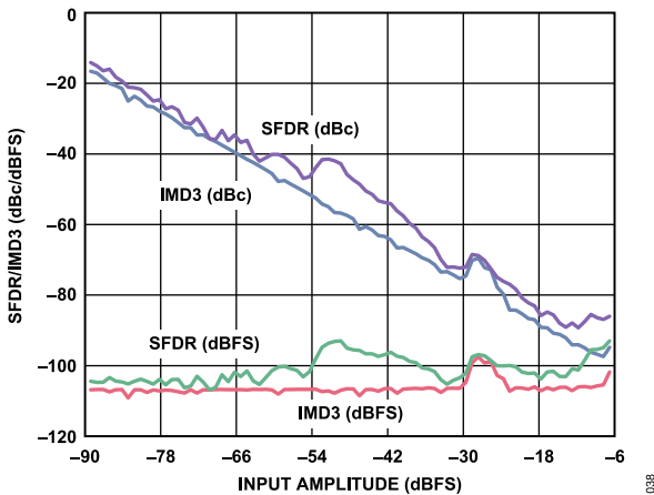
Figure 38. Two-Tone SFDR/IMD3 vs. Input Amplitude (AIN) with f_{IN1} = 70.5 \text{ MHz} and f_{IN2} = 72.5 \text{ MHz} , f_{SAMPLE} = 125 \text{ MSPS}
