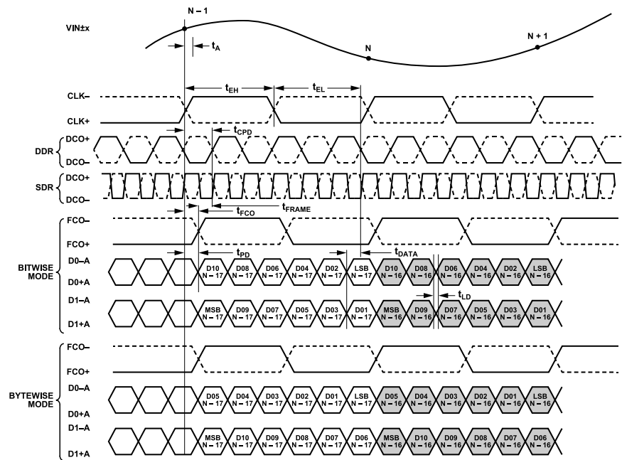
Figure 3. 12-Bit DDR/SDR, Two-Lane, 1x Frame Mode
