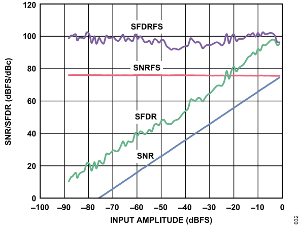
Figure 36. SNR/SFDR vs. Analog Input Level, f_{IN} = 9.7 \text{ MHz} , f_{SAMPLE} = 125 \text{ MSPS}
