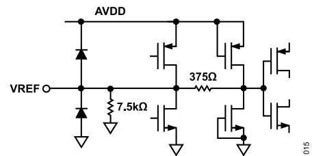
Figure 54. Equivalent VREF Circuit
