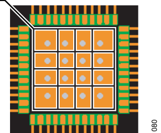
Figure 75. Typical PCB Layout
