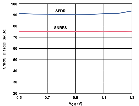
Figure 56. SNR/SFDR vs. Common-Mode Voltage, f_{IN} = 9.7 MHz, f_{SAMPLE} = 125 MSPS
