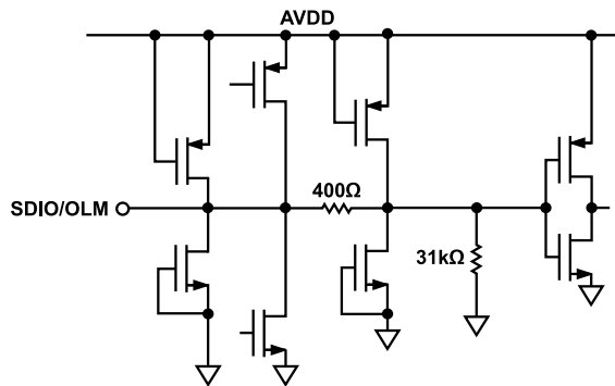
Figure 49. Equivalent SDIO/OLM Input Circuit
