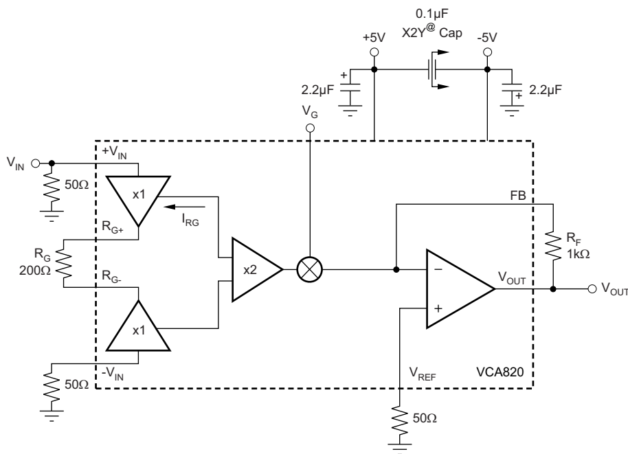
Figure 76. DC-Coupled, A_{VMAX} = 20 dB, Bipolar Supply Specification and Test Circuit
