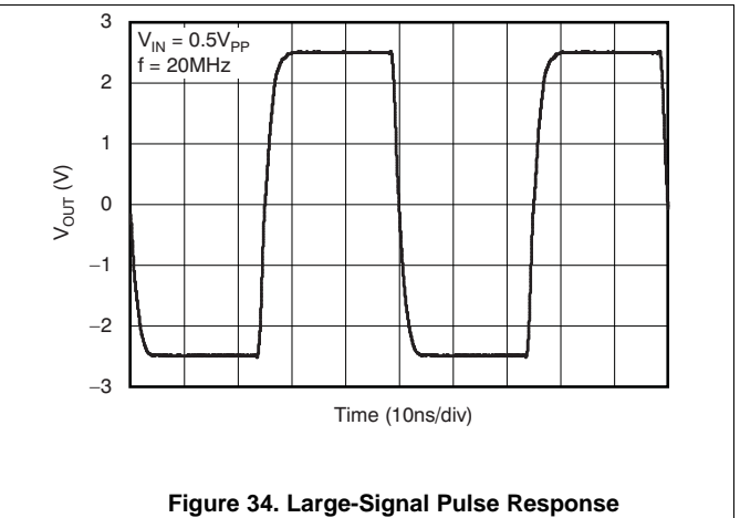
Figure 34. Large-Signal Pulse Response
