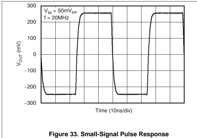
Figure 33. Small-Signal Pulse Response
