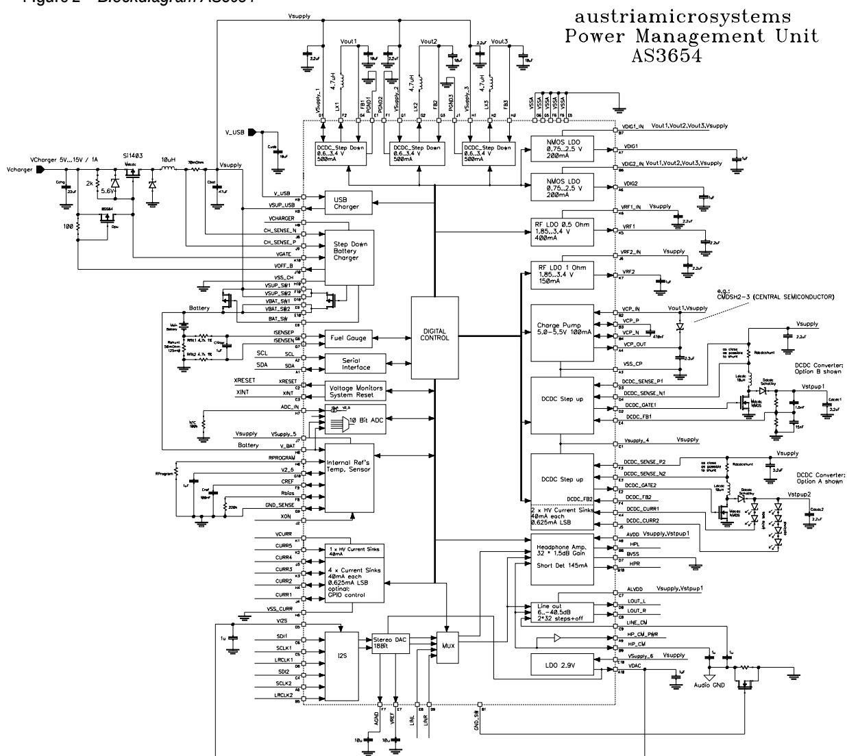
Figure 2 – Blockdiagram AS3654
