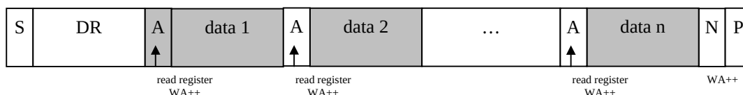
Figure 28 – I 2 C Current-Address-Read:
