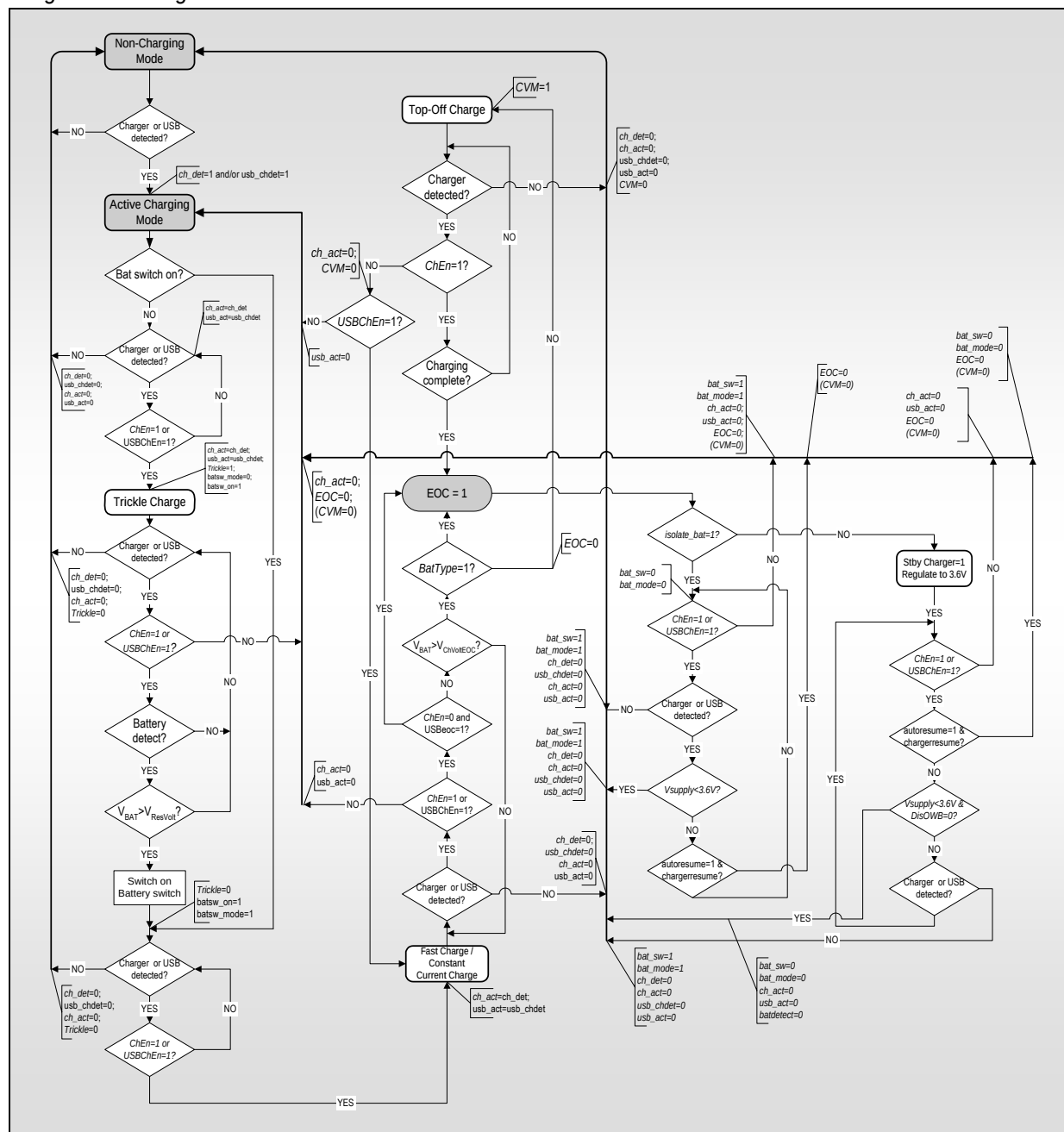
Figure 13 – Charger Flow Chart
