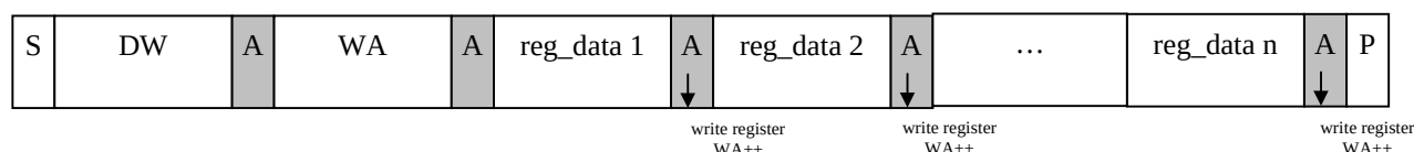
Figure 25 – I 2 C Page-Write:
