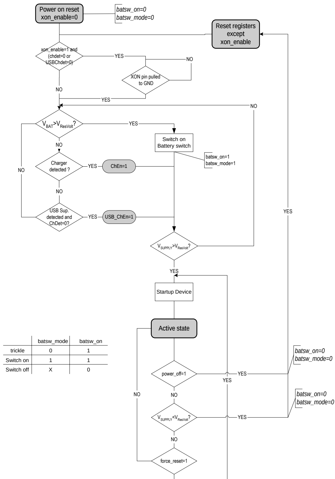
Figure 29 – Startup flow chart
