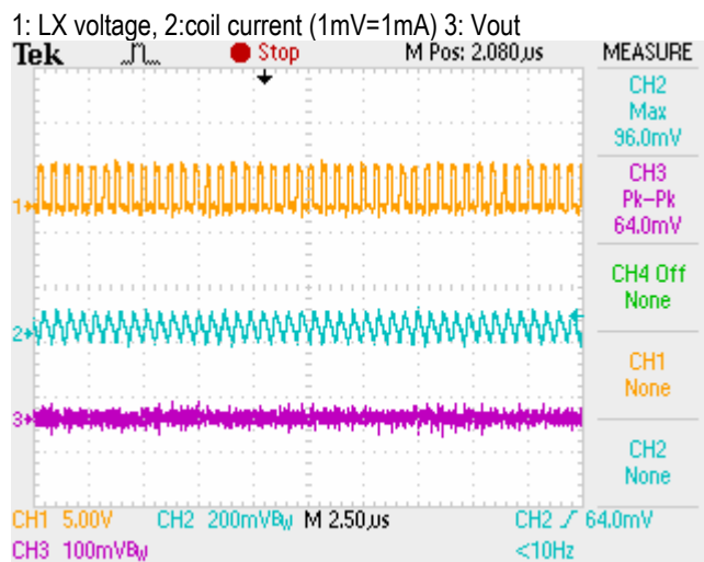
Figure 15 –sdX_dis_curmin=1 operation
