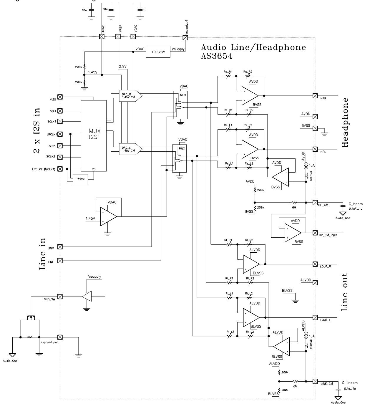
Figure 22 – Audio Blockdiagram
