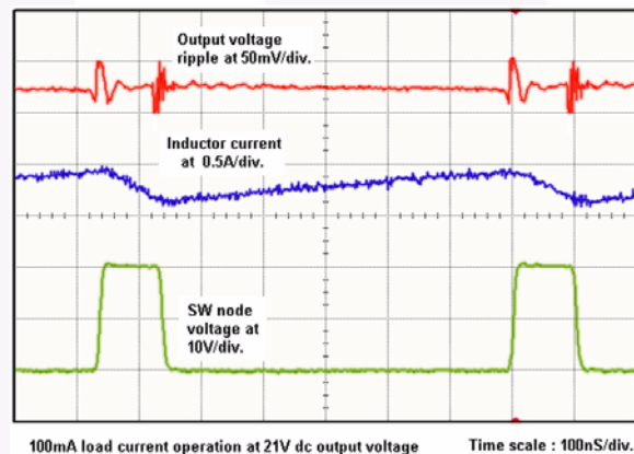
Figure 7. 100mA Load Current Operation
