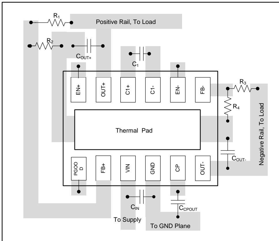
Figure 16. LM27762 Layout Example (Note: Pullup resistor for PG00 not shown in example.)
