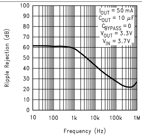
Figure 10. Ripple Rejection
