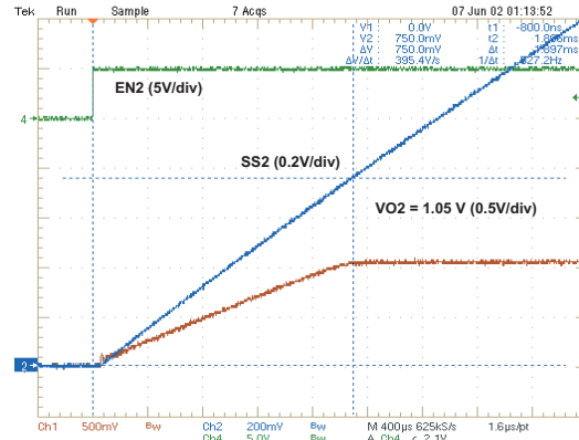
Figure 22. Start-Up Waveforms
