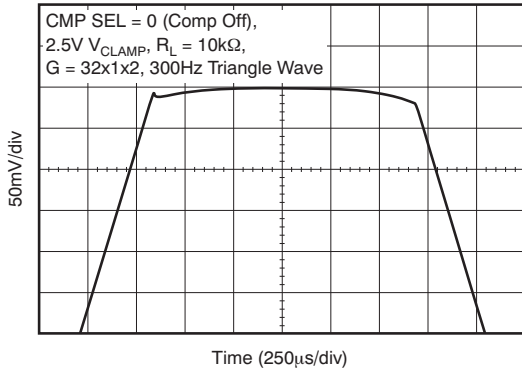
V_{CLAMP} RESPONSE ( C_L = 10\text{nF} , CMP SEL = 0)
