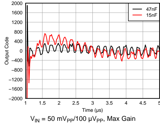
Figure 57. Overload Recovery Response vs INM Capacitor (Zoomed)
