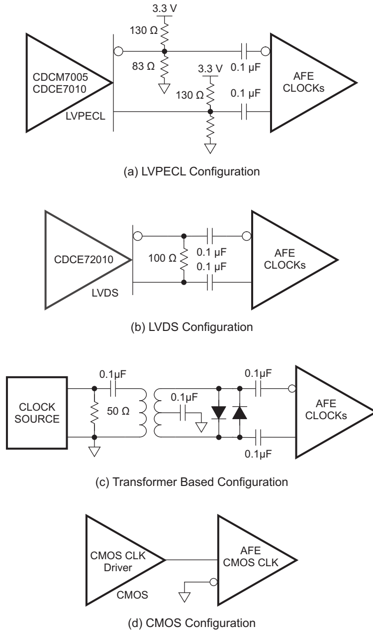
Figure 88. Clock Configurations
