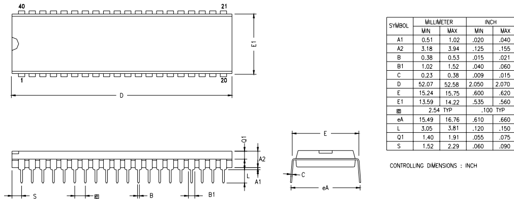
Figure 103. 40-Lead Plastic Dual-Inline Package (PDIP)
