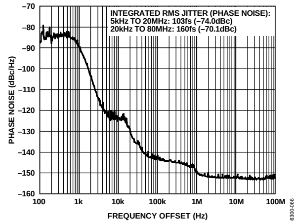
Figure 5. Absolute Phase Noise (Output Driver = LVPECL), f_{REF} = 19.44 MHz, f_0 = 311.04 MHz, LBW = 1 kHz, f_{SYSCLK} = 1 GHz, PLL Off
