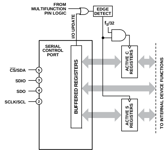
Figure 66. Buffered and Active Registers
