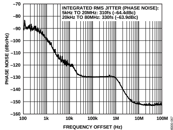
Figure 6. Absolute Phase Noise (Output Driver = LVPECL), f_{REF} = 19.44 MHz, f_0 = 311.04 MHz, LBW = 1 kHz, f_{SYSCLK} = 50 MHz (Crystal), PLL On
