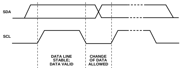
Figure 60. Valid Bit Transfer
