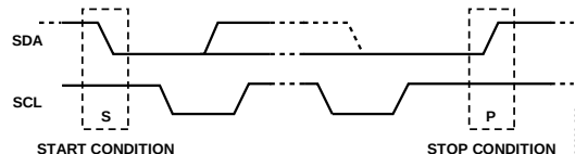
Figure 61. Start and Stop Condition
