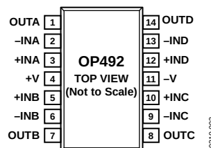
Figure 2. 14-Lead Narrow-Body SOIC (S-Suffix)
