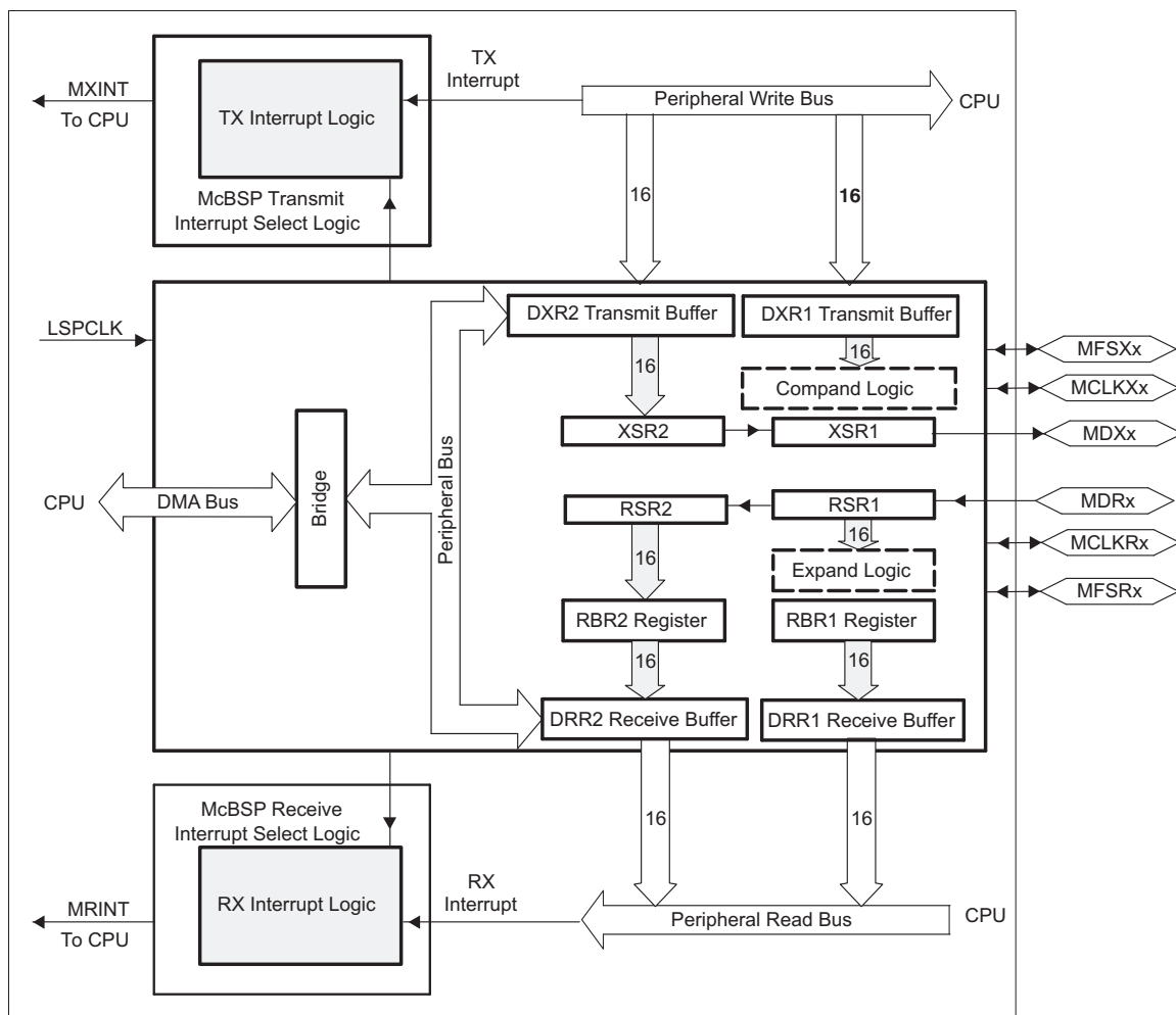
Figure 6-11. McBSP Module
