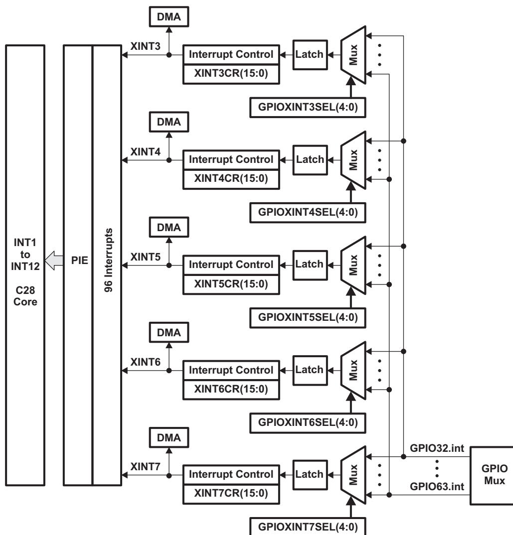
Figure 6-27. External Interrupts
