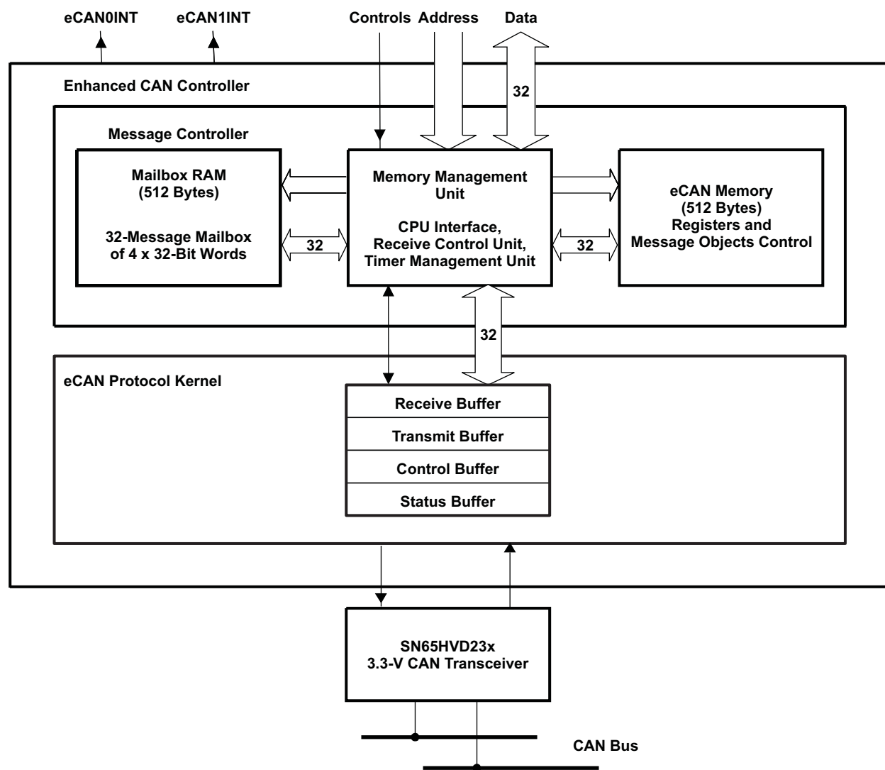
Figure 6-12. eCAN Block Diagram and Interface Circuit
