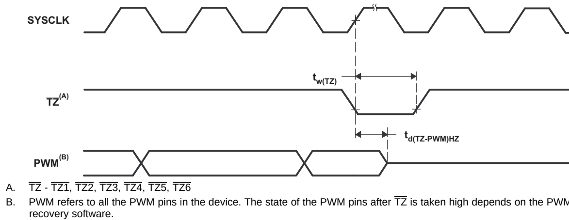
Figure 5-14. PWM Hi-Z Characteristics
