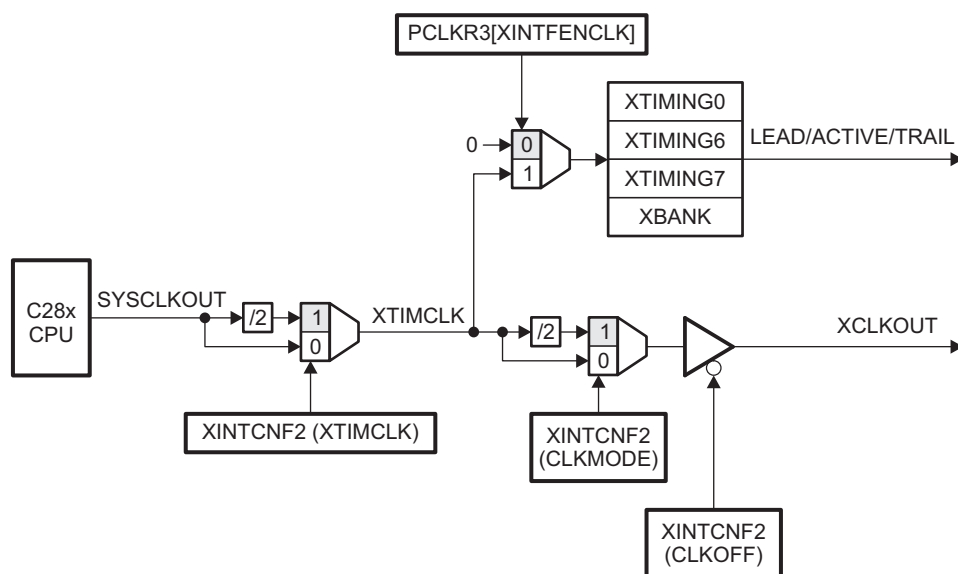
Figure 5-28. Relationship Between SYCLKOUT and XTIMCLK
