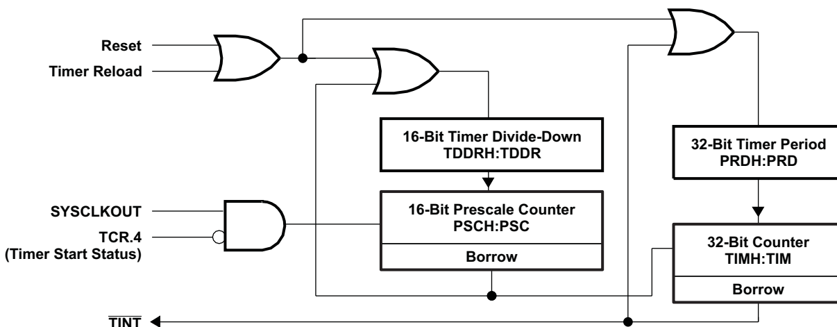
Figure 6-2. CPU-Timers
