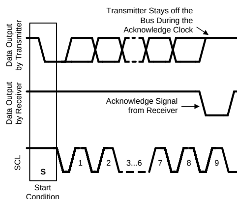
Figure 21. Acknowledge Signal
