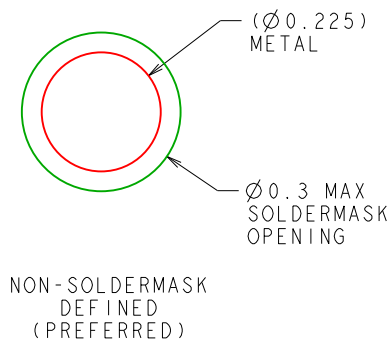
SOLDERMASK DETAILS NOT TO SCALE
