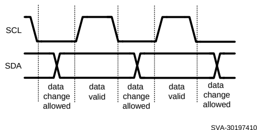
Figure 20. Data Validity
