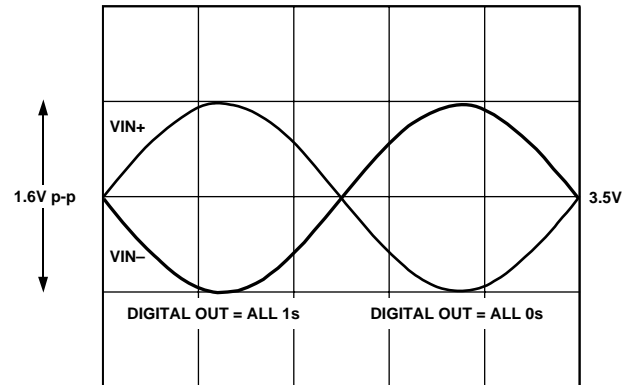
Figure 57. Differential Analog Input Range for VREF = 1.6 V
