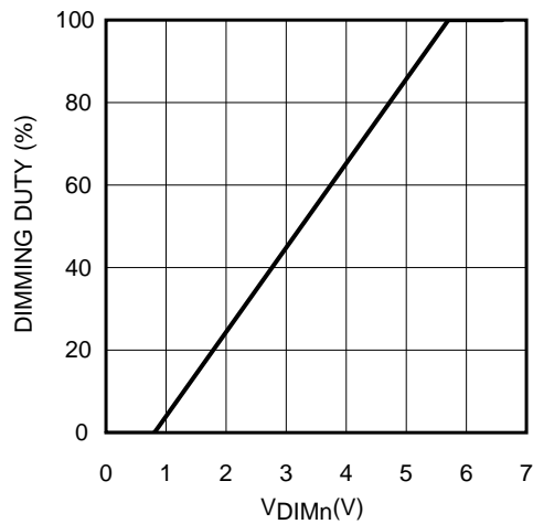
Figure 34. Dimming Duty vs V DIMn in DC interface mode
