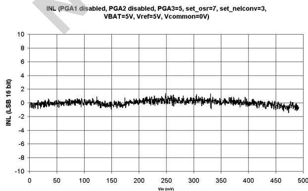
Figure 16-11. Integral non-linearity of the ADC and gain of 5 (PGA1 and PGA2 disabled, PGA3=5, reference voltage of 5V)
