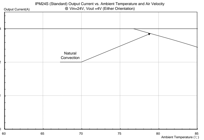
Figure 35: Output current vs. ambient temperature and air velocity Vin=24V, Vout=4V(Either Orientation)
