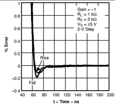
Figure 38. Settling Time
