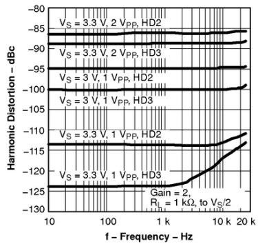
Figure 39. Harmonic Distortion vs Frequency
