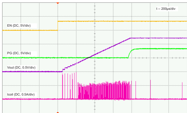
Figure 9-12. Start-Up, Load = Open
