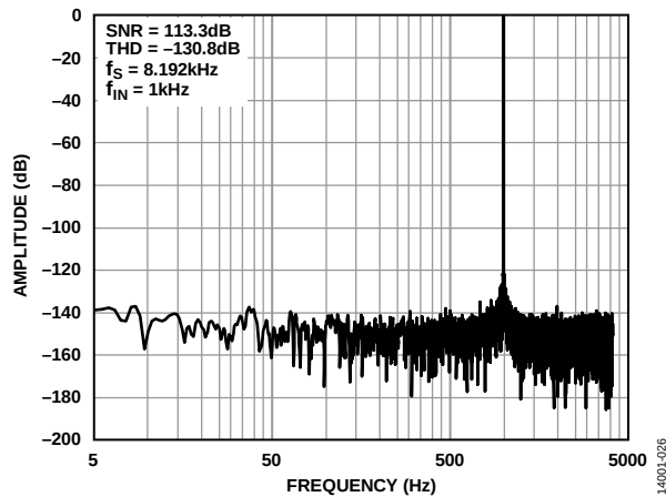
Figure 24. FFT One-Shot-Mode, Sinc5 Filter, Median Mode, Decimation = \times 64 , -0.5\text{ dBFS} , SYNC_IN Frequency = MCLK/4000
