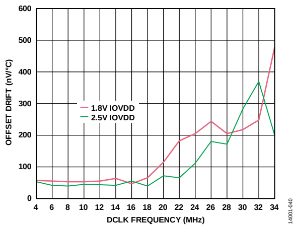
Figure 49. Offset Drift vs. DCLK Frequency
