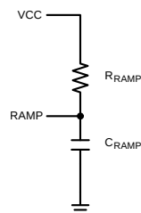
Figure 23. Additional Slope Compensation for V_{OUT} > 5\text{ V}
