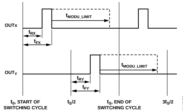
Figure 67. Setting Modulation Limits
