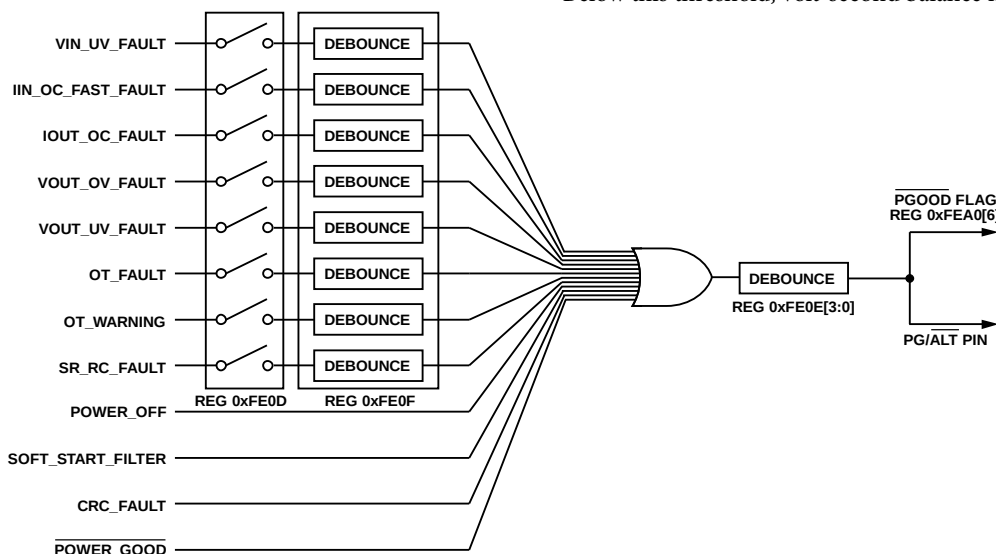
Figure 30. PGOOD Programming
