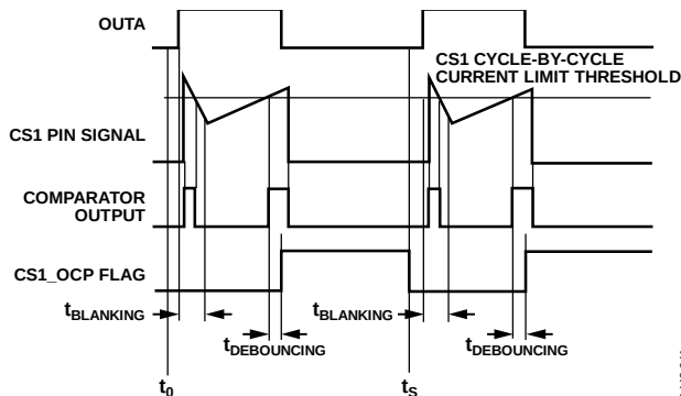
Figure 40. CS1 Cycle-by-Cycle Current-Limit Timing
