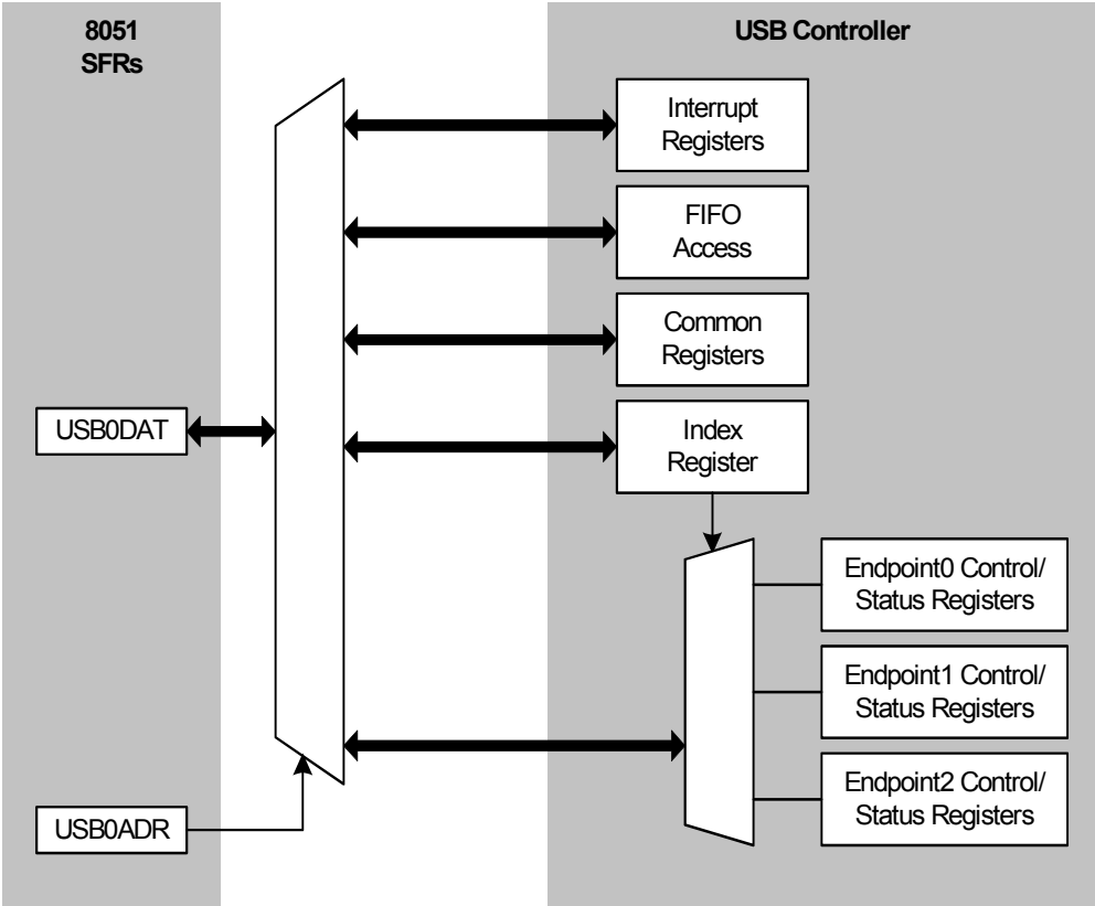
Figure 18.2. USB0 Register Access Scheme
