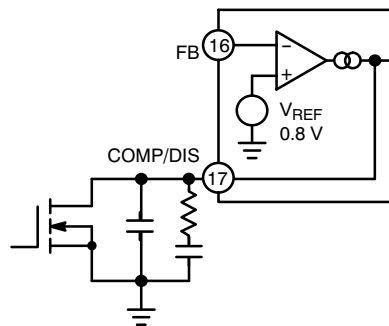
Figure 12. Disable Circuit
