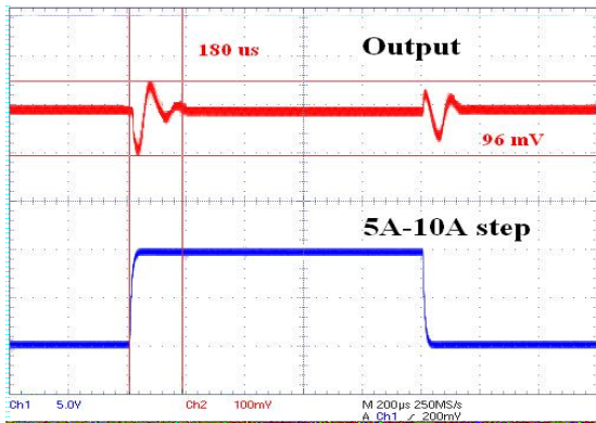
Figure 24. Transient Response ( V_{in} = 12\text{ V} , V_{out} = 3.3\text{ V} , I_{out} = 5\text{ A} to 10\text{ A} Step) Output Capacitors: 2x MLCC 100 µF and 820 µF OS-CON
