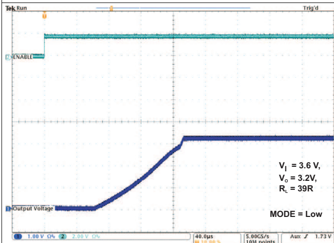
Figure 25. TPS82699 Start-Up
