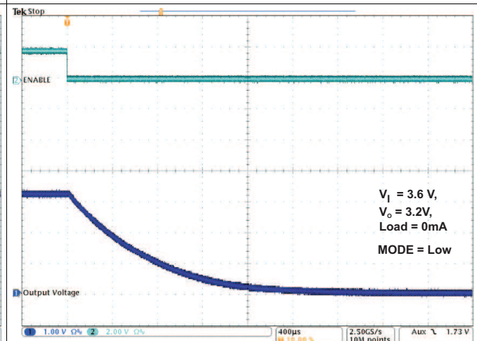
Figure 26. TPS82699 Shutdown
